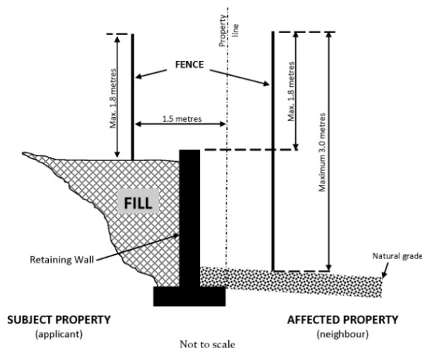
Diagram 4.17.3 : FENCE PLACEMENT
