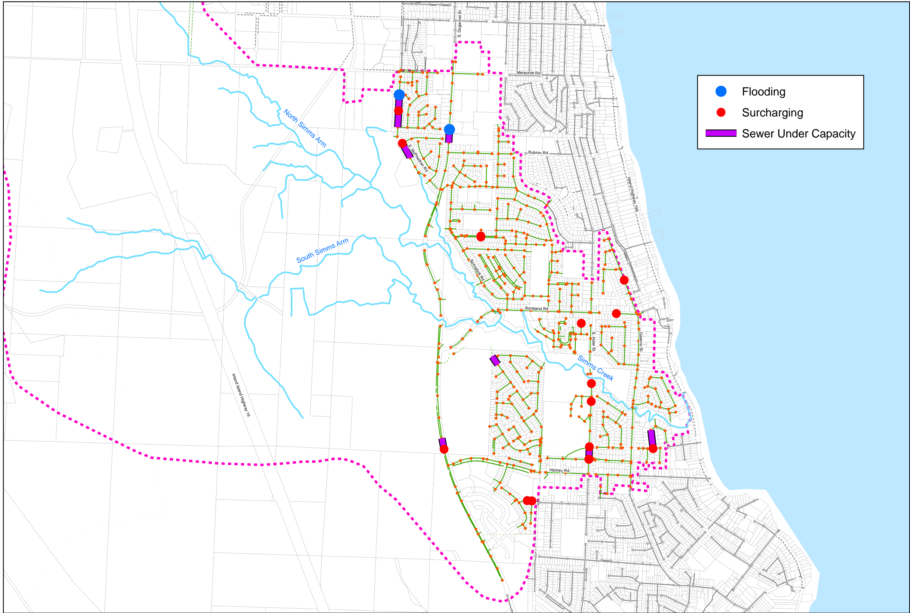
Simms Creek Watershed Municipal Drainage System Modeled Deficiencies (Existing Conditions)
