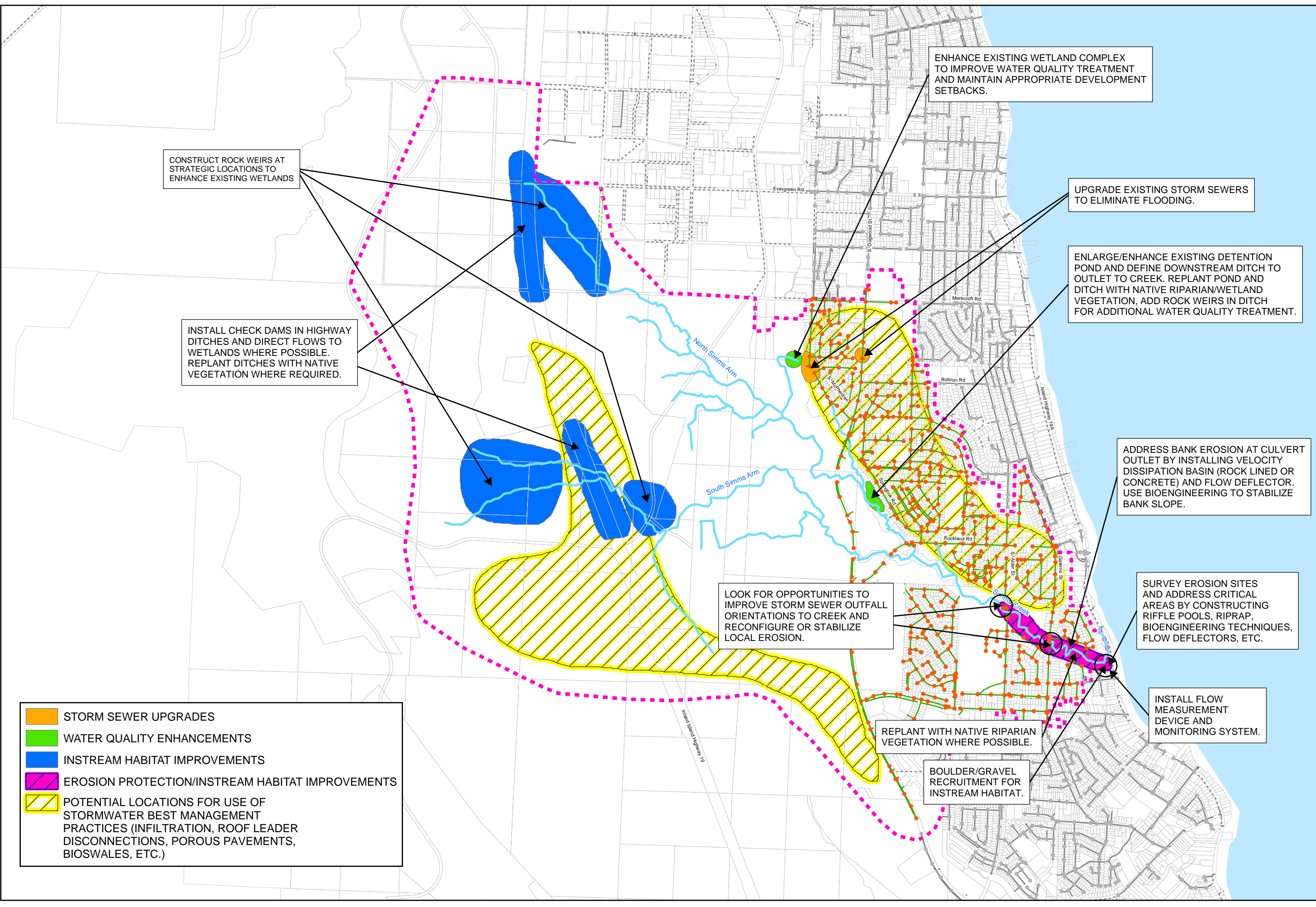
Figure 10.1 Simms Creek Watershed Recommended Works
