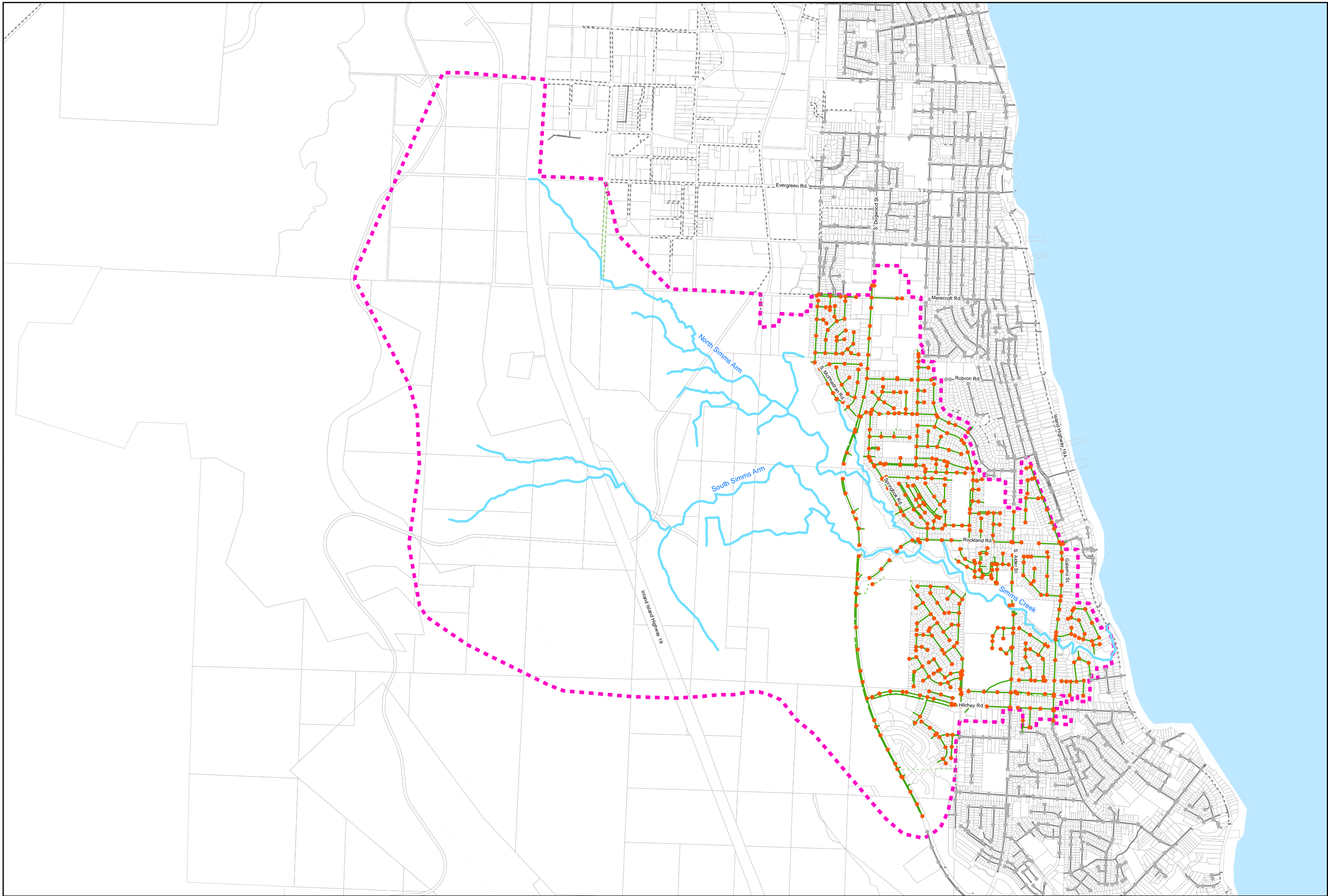
Figure 3.3 Simms Creek Watershed Municipal Drainage System
