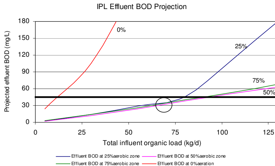
FIGURE 3.11 IPL EFFLUENT BOD PROJECTIONS WITH AERATION
